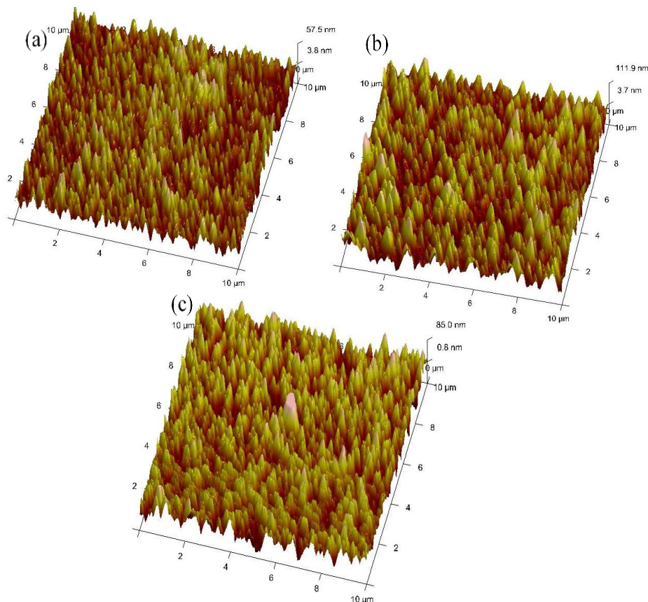
Fig. 4 3D AFM images of b-Si wafers formed after etching c-Si with Ag NPs of different morphology resulted from Ag thin films of different thicknesses; (a) 10 nm (b) 15 nm and (c) 25 nm.
