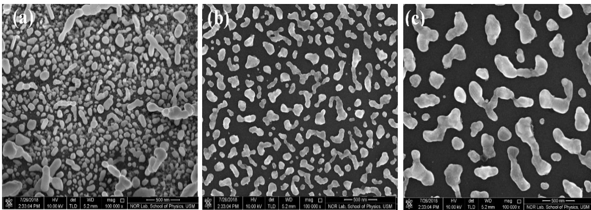
Fig. 1 30° tilt top view FESEM images of wafers with Ag NPs formed after annealing c-Si with Ag thin films of different thicknesses at 240°C for 40 min under \text{N}_2 ; (a) 10 nm (b) 15 nm and (c) 25 nm. The scale bar represents 500 nm.
